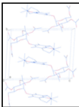
Fig. 2. The packing diagram viewed along a axis. Only non-hydrogen atoms are shown.
